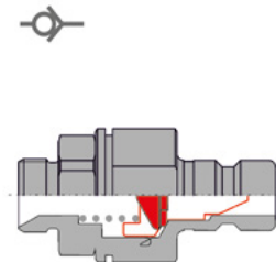
Self-sealing coupling = coupling with valve
